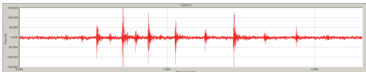
Figure 10. Pressure waveform for “popping” noises.
