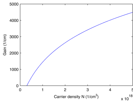
Figure 4.14 Gain model. Logarithmic material gain model, which we use with traditional rate equations for further laser analysis.
