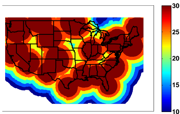
Figure 12: Estimate of the SNR of the strongest Loran signal.
