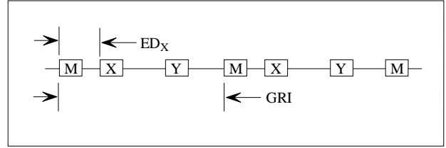
Figure 3: Loran chain Emission Delay.
