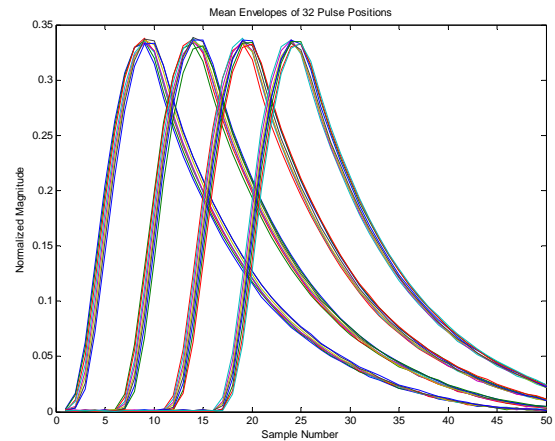
Figure 32: Received Loran pulse envelopes.
