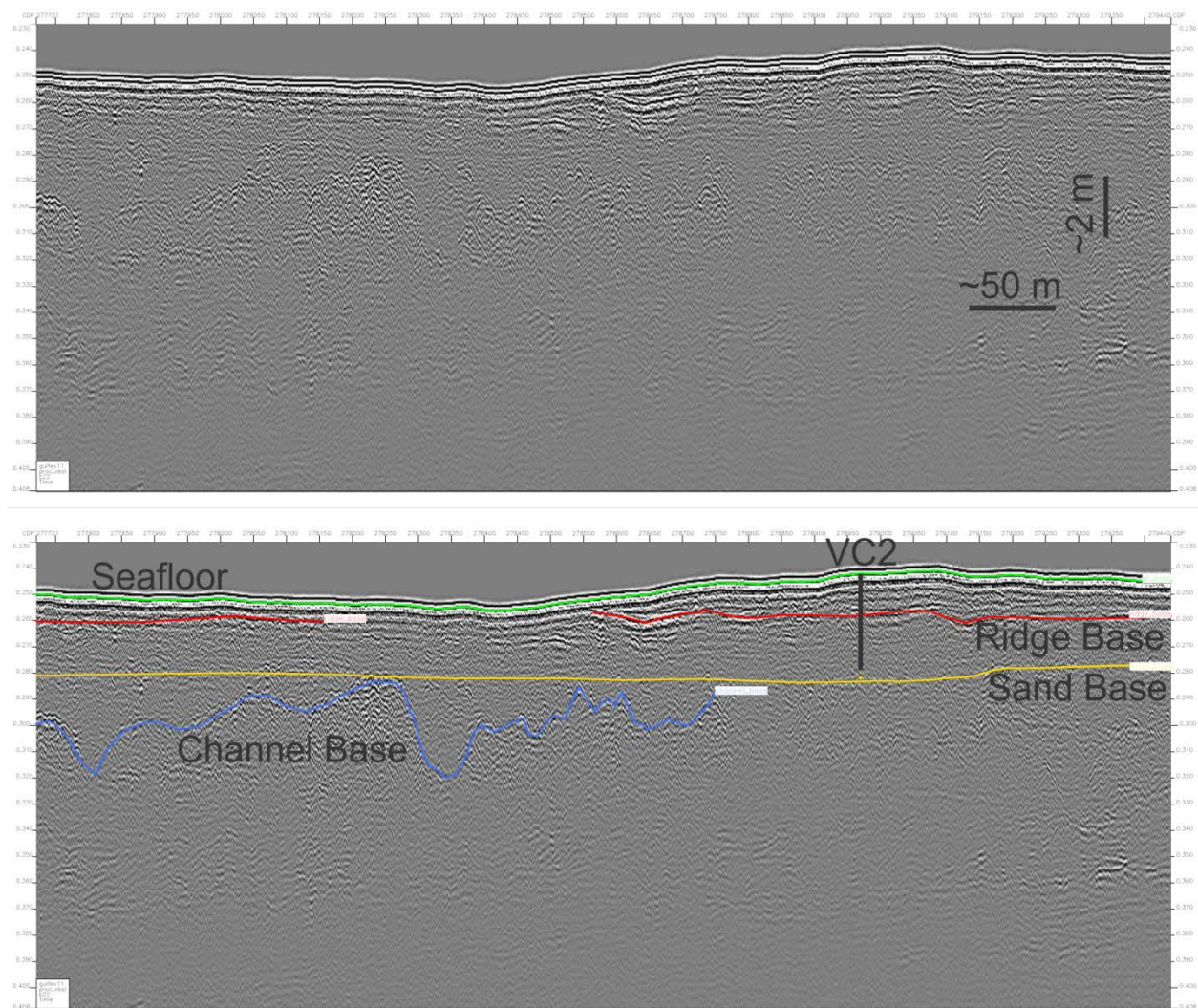
Figure 5. Uninterpreted (top) and interpreted (bottom) CHIRP section demonstrating primary stratigraphic elements of the shallow subsurface in the vicinity of core VC2. The depth of penetration of VC2 is indicated by the vertical black line on the bottom panel.
