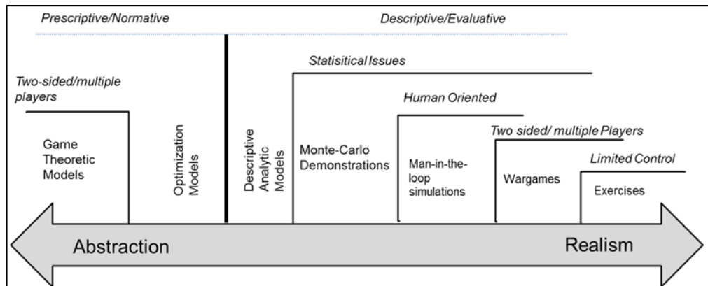
Figure 4. Modeling spectrum; from Washburn and Kress.
