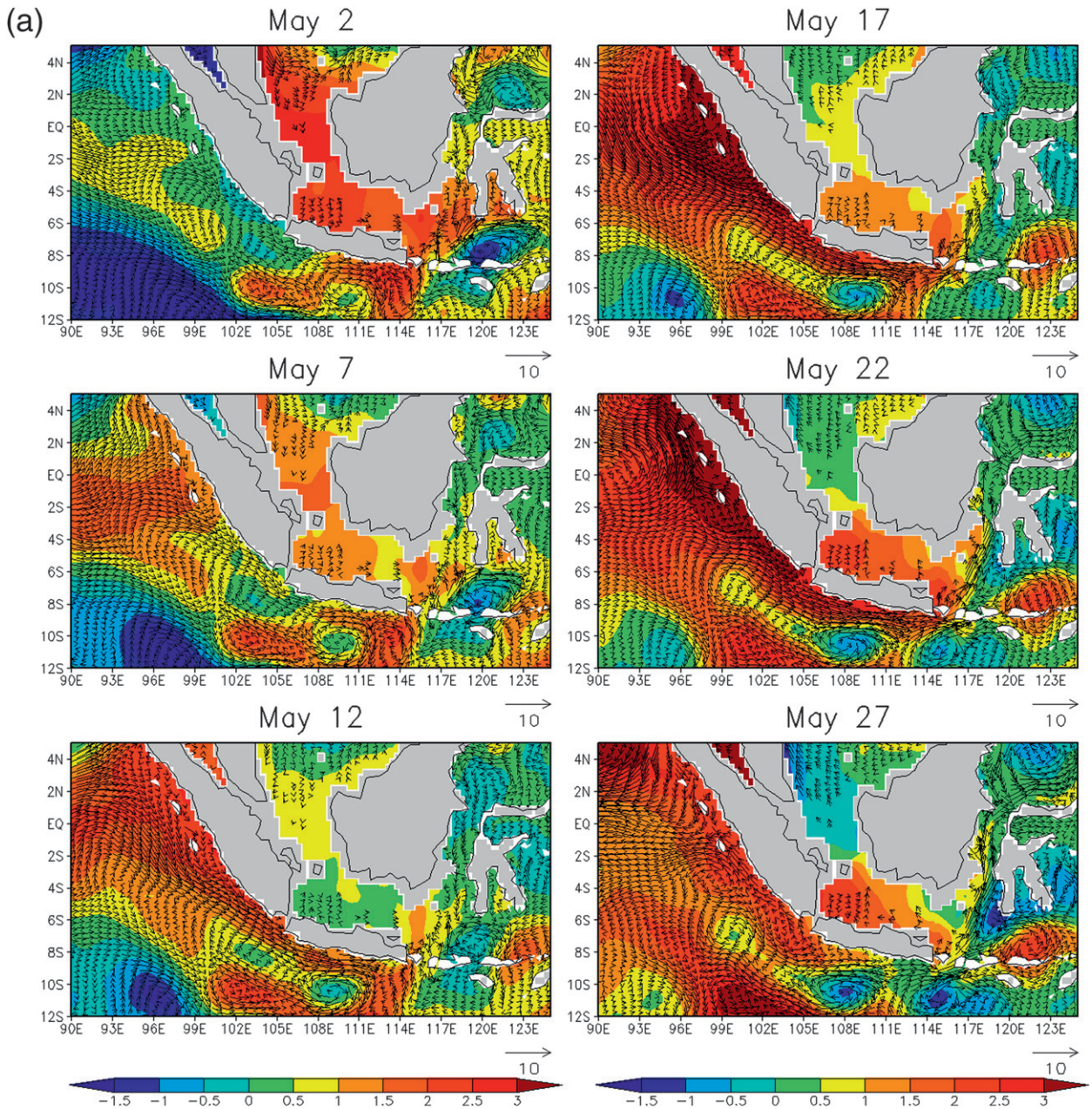
FIG. 5. (a) Anomaly snapshots of SSH (shading, cm) and upper-ocean (average over 50–150-m depth) velocity (vectors, \text{cm s}^{-1} ) from the annual cycle relative to the April–June mean derived from the Indo-Pacific basin HYCOM simulation. The snapshots cover 2–27 May. Gray shading indicates land grid points in the model. (b) As in (a) but for SSH (shading, cm) anomalies from satellite altimeter data and wind stress (vectors, \text{N m}^{-2} ) anomalies used to force the model. The color scale is different from (a). (c) SSH (shading; m) and upper-ocean (average over 50–250-m depths) velocity (vectors) anomalies during 9–30 May 2004 relative to the mean of April–June 2004 from the global HYCOM simulation. A 30-day running filter has been applied to the time series. (d) As in (c) but for a smaller domain and the period 17–27 May 2004. (e) Alongshore and along-strait velocity (shading) and SSH (contour) anomalies along the gray solid line shown in Fig. 1. Both alongshore and along-strait velocities are defined as the velocity component along the gray line. Contour interval is 0.5 cm; the dashed contour line indicates negative values and blue solid lines indicate the phase line of 2.5 \text{ m s}^{-1} .
