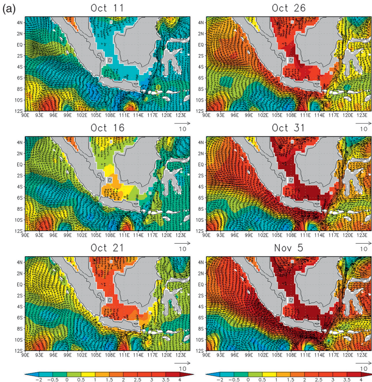
FIG. 7. (a),(b) As in Figs. 5a,b but for the period 11 Oct–5 Nov 2005 and anomalies are relative to the October–November mean. (c) As in Fig. 5c but for the period 29 Oct–19 Nov 2005 and anomalies are relative to the October–November mean. White lines are the same as the gray lines in Fig. 1a. (d) As in Fig. 5d but for the period 8–18 Nov 2005. (e) As in Fig. 5e but for the period 5 Oct–11 Dec 2005.
