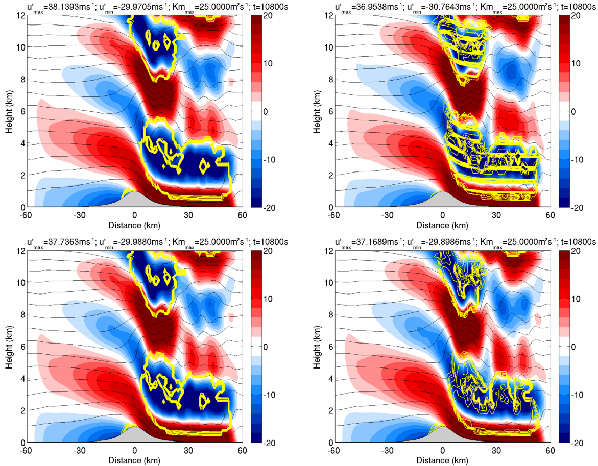
Figure 3: Perturbed u -component of the wind (filled contours, c.i. 2 \text{ ms}^{-1} ), potential temperature (black lines, c.i. 10 \text{ K} ), mixing coefficient (yellow contours, c.i. 5 \text{ m}^2\text{s}^{-1} ) and the mountain (gray). Plots are for the effective grid scale being node-specific (top left), node-specific, limited by the vertical nodal spacing (top right), element-averaged (bottom left) and element-averaged, limited by the average vertical nodal spacing (bottom right).
