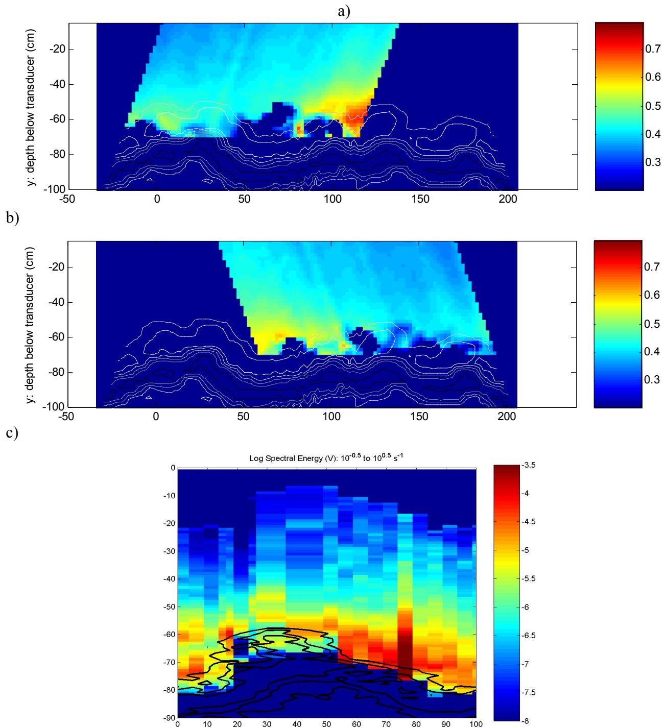
Figure 5: Near-bed flow variability as inferred from 9/04 ADCP (a and b) and 8/04 BCDV (c) RBP deployments. ADCP data shows beam velocity standard deviations within the plane of wave motion (on- offshore) for a region near the bed. Contours indicate ADCP correlation magnitude from which bed morphology can be inferred. BCDV-derived spectral energy is indicative of near-bed turbulence surrounding a coral head. Contours here indicate acoustic backscatter levels. The profile in (c) is displaced approximately 20 cm laterally(along-shore) from the profiles in (a) and (b). The horizontal axis indicates cross-shore position, consistent for the 3 panels.
