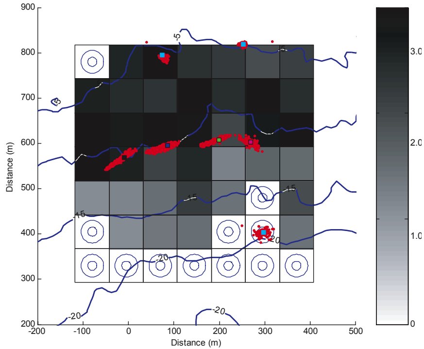
Figure 3: Spectral roughness energy (expressed as RMS height in cm) for the 63-100 cm band from boat-based altimetry surveys. Boxes with insufficient data are shown with targets. Current scatter data from July 2004 experiment are overlaid. Sites AF, C1, C2 and C3 (see figure 2) show greater scatter since these are near-bed velocities. Bathymetry contours at 5m intervals are also shown.
