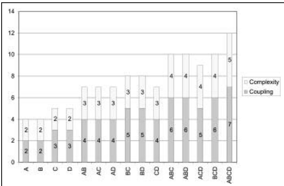
Figure 2: Metrics for Program Slices
