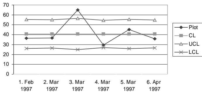
Figure 3. Control Chart for Code Peer Review Defects
