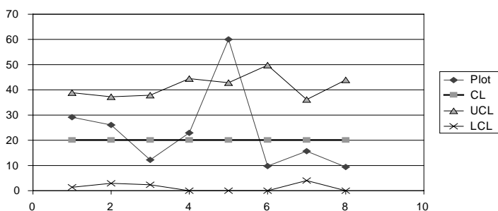
Figure 4. Control Chart for Code Peer Review Defects
