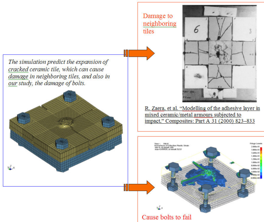
Figure 8. Ballistic impact on armor cause damage in bolts and neighboring tiles
