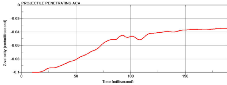
Figure 11. The changing velocity of projectile with time
