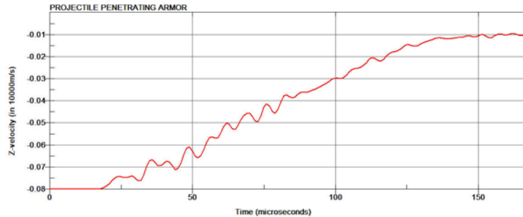
Figure 7. Change of projectile velocity with time
