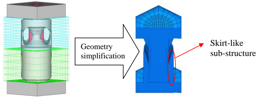
(a) design from topology optimization tools (b) modified design (cut in half to show the cross section shape)
