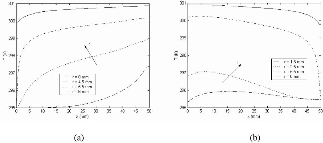
Figure 8- Variations of temperature profile in the radial position ( q_w'' = 30kW / m^2 , \Delta T_{sub.li} = 5K , \lambda_{eff} = 10W / m \cdot K , \Delta P_{ext} = 40kPa ): (a) circular core and (b) annular core
