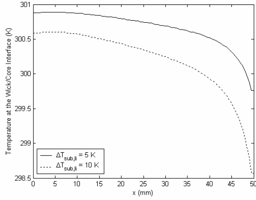
Figure 12- Influence of inlet liquid sub-cooling on temperature at the wick/core interface ( q_w'' = 30kW / m^2 , \lambda_{eff} = 10W / m \cdot K , \Delta P_{ext} = 40kPa )
