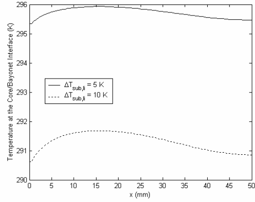
Figure 13- Influence of inlet liquid sub-cooling on temperature at the core/bayonet interface ( q_w'' = 30kW / m^2 , \lambda_{eff} = 10W / m \cdot K , \Delta P_{ext} = 40kPa )
