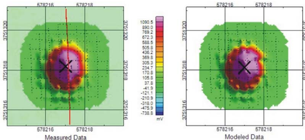
Figure 3-7. Example of a measured EM61-MK2 data chip of an anomaly (left) and the corresponding model result (right). The axes labels refer to distance in meters.
