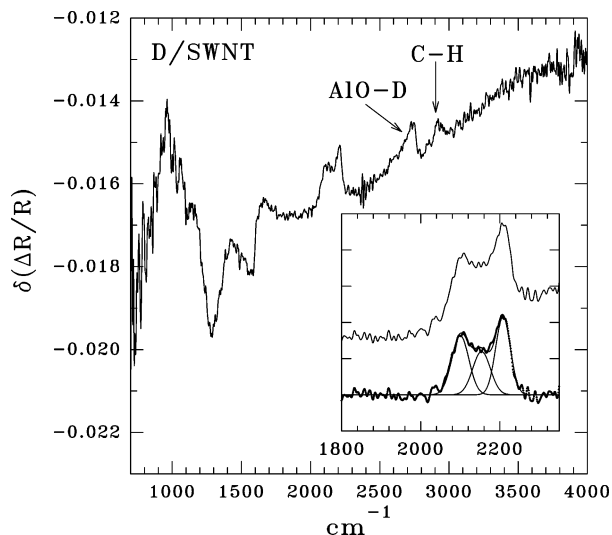
Figure 4. Similar to Figure 3 but showing the results for adsorption of D atoms. The AIO–D stretching mode, due to D adsorption on the substrate oxide, is indicated.
