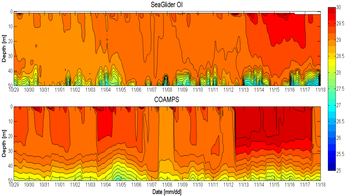
Figure. Temperature in upper 50m of the ocean. Comparison between in-situ SeaGlider observations (upper panel) and COAMPS simulation (lowe panel)
