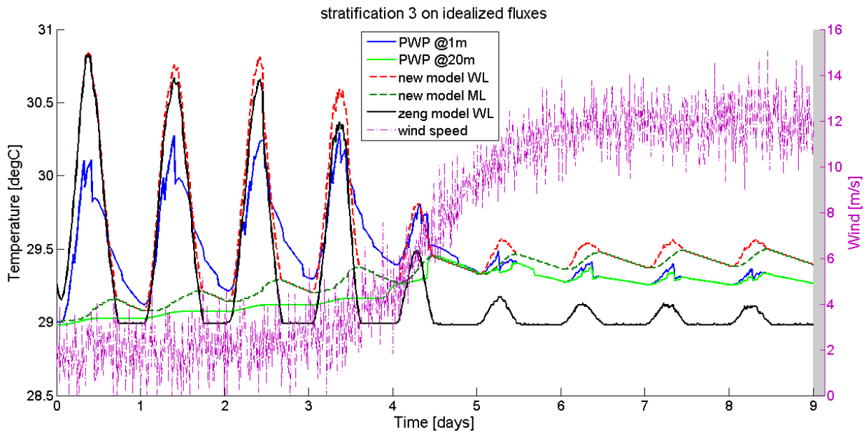
Figure. Initial validation of the model against the DYNAMO dataset shows good fidelity of the model in comparison with more complex schemes and observations.
