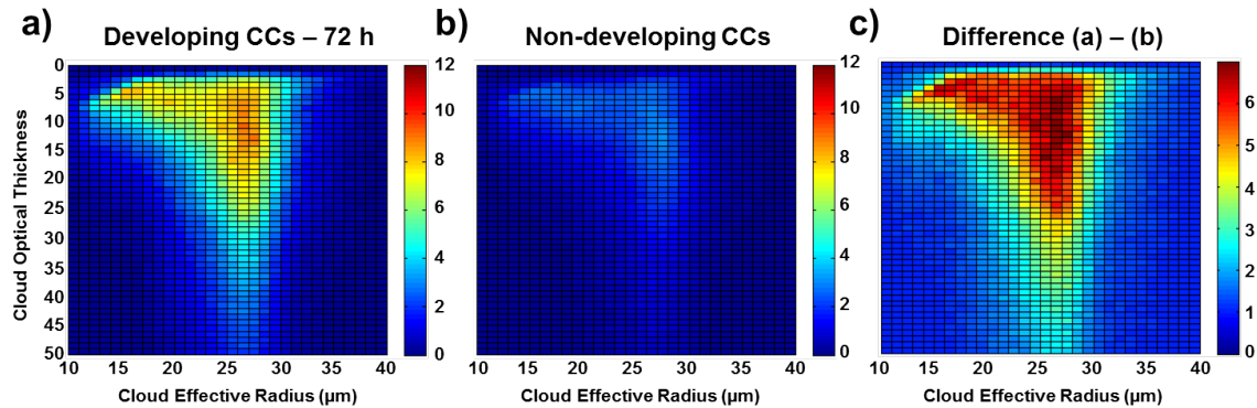
Figure 3: Cloud effective radius versus cloud optical thickness normalized frequency plots for a 72-h period for: a) developing cloud clusters; b) non-developing cloud clusters; and c) the difference between the two.
