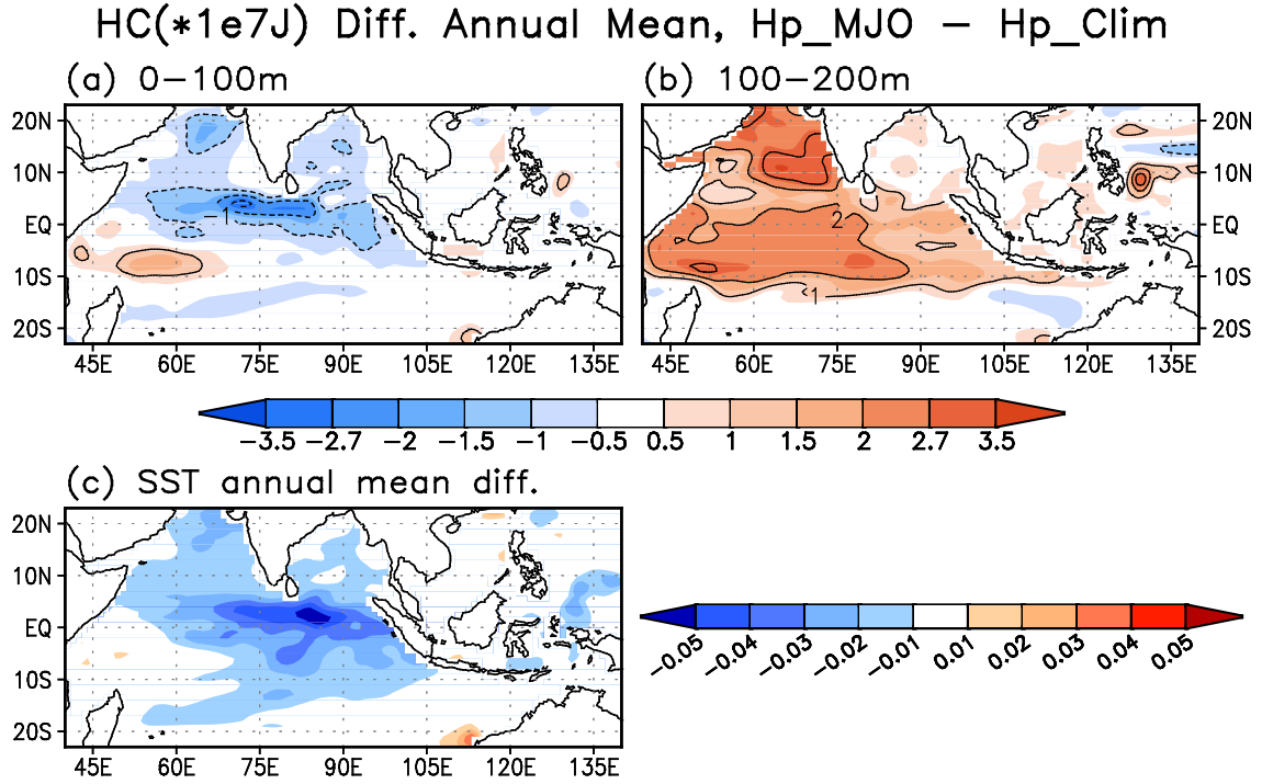
Figure 10. Annual mean difference in heat content between the Hp_MJO and Hp_Clim simulations (a) for upper 100m, and (b) 100–200m. Unit is 10^7\text{J/m}^2 . (c) Annual mean difference of SST ( ^{\circ}\text{K} ).
