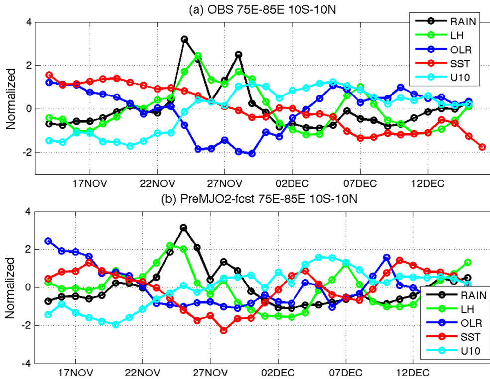
Figure 5. Normalized time-series averaged over the area 75^{\circ}\text{E} - 85^{\circ}\text{E} , 10^{\circ}\text{S} - 10^{\circ}\text{N} from (top) observations and (bottom) model, showing (black) rainfall, (green) latent heat flux, (blue) OLR, (red) SST, and (cyan) 10-m zonal wind speed.
