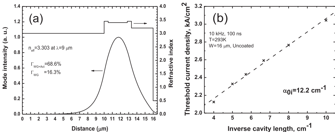
FIG. 5. (a) \text{TM}_{00} waveguide mode and waveguide refractive index profiles in our devices. (b) Dependence of the threshold current density in our devices on the reciprocal cavity length. The value of waveguide loss of \alpha_{0i} \approx 12.2 \text{ cm}^{-1} is obtained assuming J_{th}(1/L) \propto \alpha_{tot} = \ln(R_m)/L + \alpha_{0i} , where R_m \approx 0.28 is the uncoated facet reflectivity and L is the laser cavity length.
