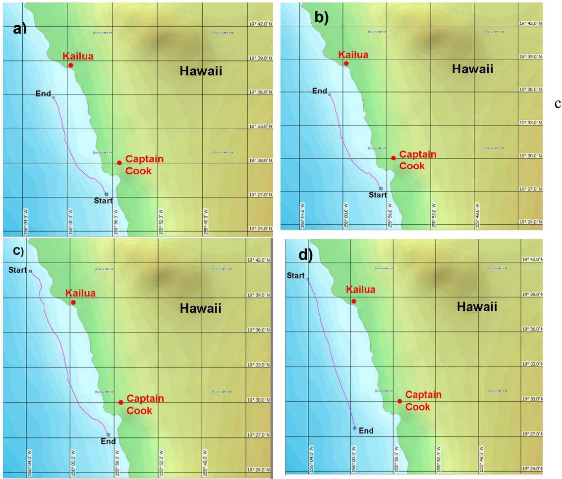
Fig. 3a-d. EK-60 survey lines. Fig. a and c are the shallow transect with depth varying from 500-700m. Fig. b and d are the deep transects with depth varying from 1100-1300m. Fig. a and b are the South to North survey beginning south of Captain Cook, HI and ending near Kailua-Kona, HI. Fig. c and d are the North to South survey beginning north of Kailua-Kona, HI and finishing south of Captain Cook, HI.
