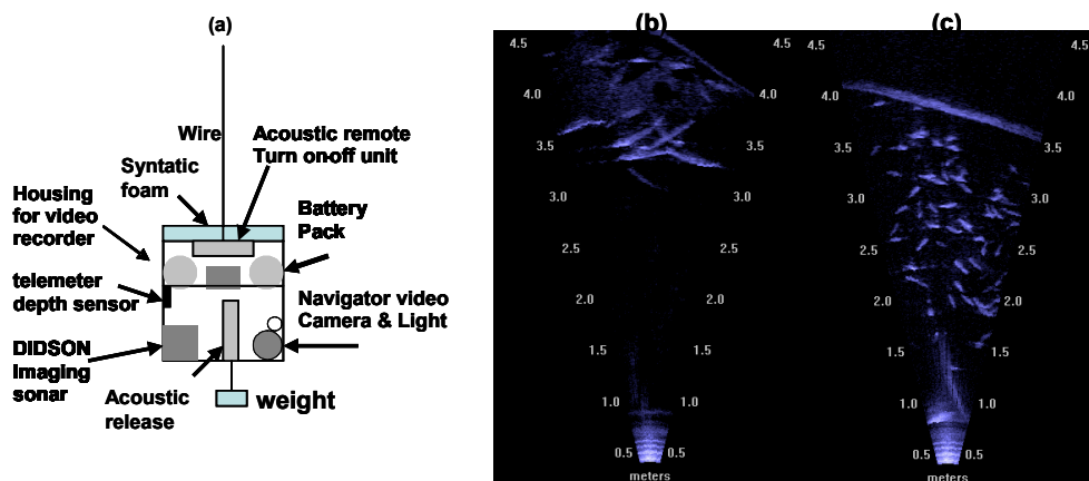
Figure 1. (a) schematic of a profiler to examine the micronektons in the deep layers that beaked whales forage in, (b) DIDSON images of pink snappers having lengths of (b) 38 – 50 cm, (c) 10 – 15 cm.
