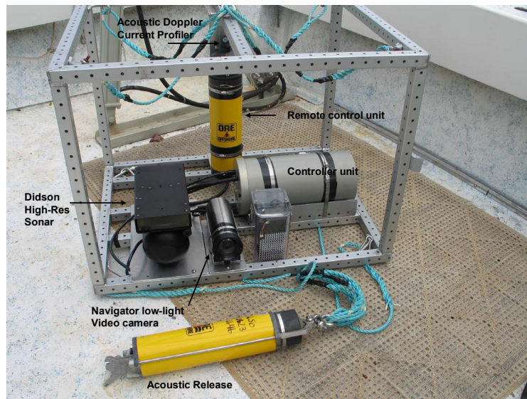
Figure 4. A photograph of the partially constructed profiler. Syntactic foam blocks will be attached to the topside of the profiler to provide floatation and weights will be attached to the acoustic release to provide negative bouyance. Batteries will be contained in the controller unit along with a digital tape recorder.
