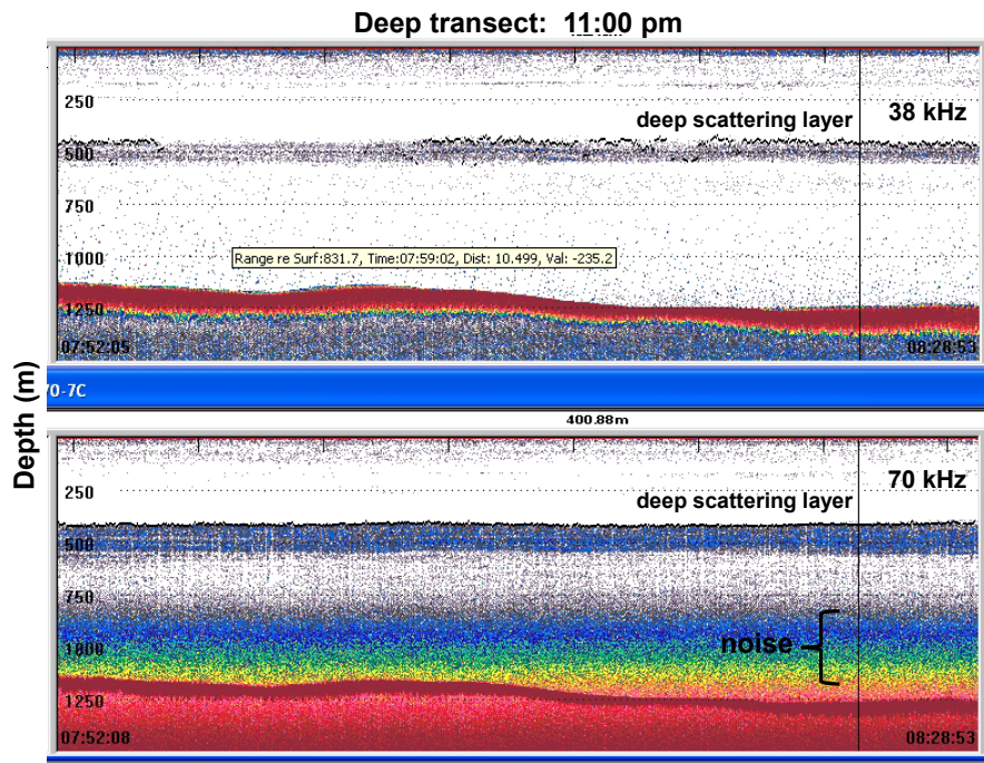
Figure 8. EK-60 echograms during the deep-water transect at 11:00 pm. The horizontal distance travel by the boat was approximately 3 km.
