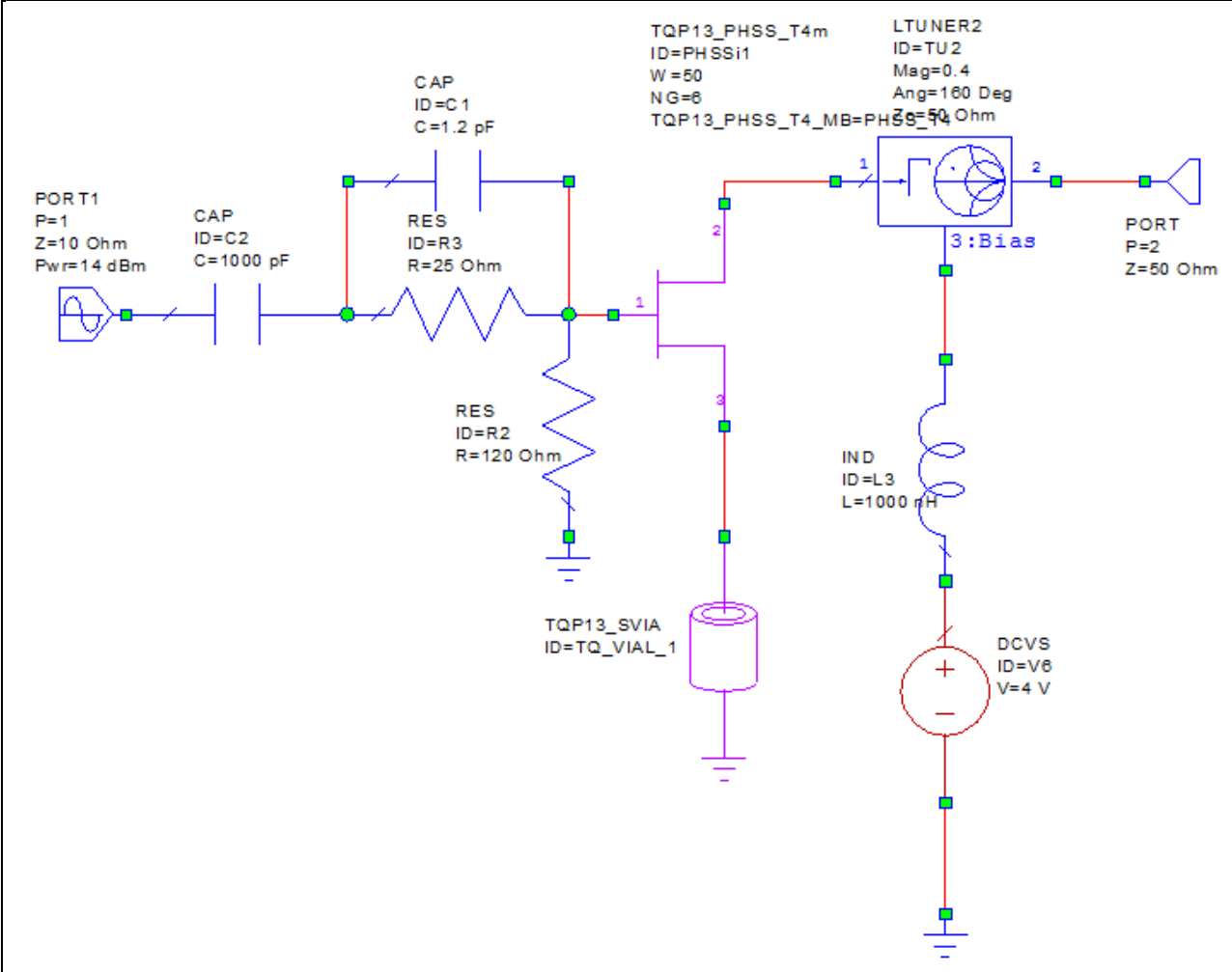
Figure 25. Schematic of the stabilized 6x50 μm PHEMT for a 28-GHz amplifier load-pull simulation.
