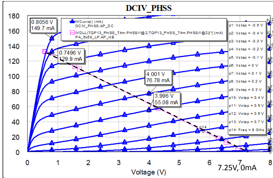
Figure 1. DC I-V characteristics of 6x50 \mu m PHEMT (TQP13 process).
