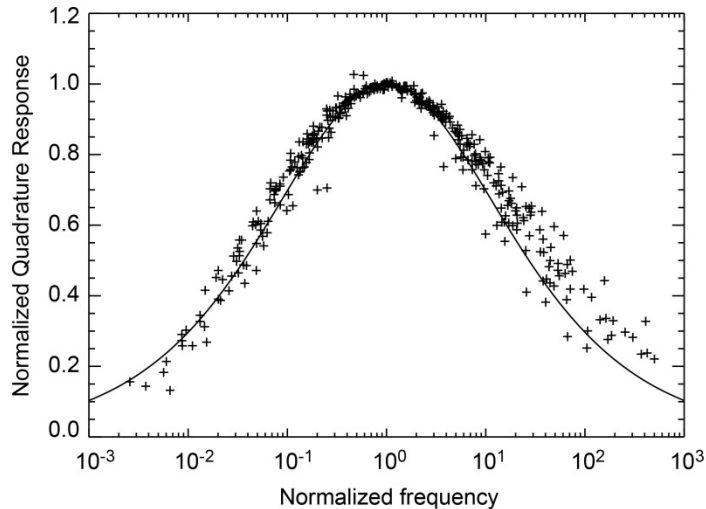
Figure 5. Comparison of quadrature response for a variety of compact steel targets with the magnetic surface mode function given by equation (16).
