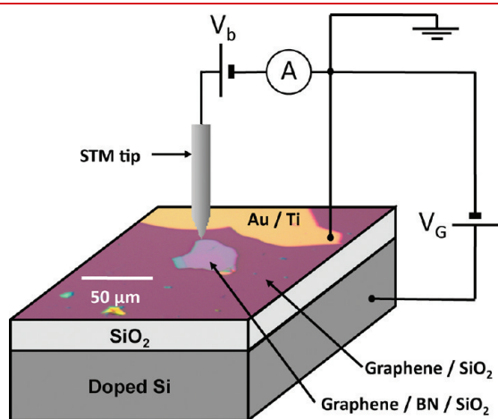
Figure 1. Optical image of graphene/BN device integrated into STM. A CVD-grown graphene layer is mechanically placed over a BN flake set upon a SiO 2 substrate. The graphene is grounded via a gold/titanium electrode. A back-gate voltage V_G is applied to the doped Si electrode.
