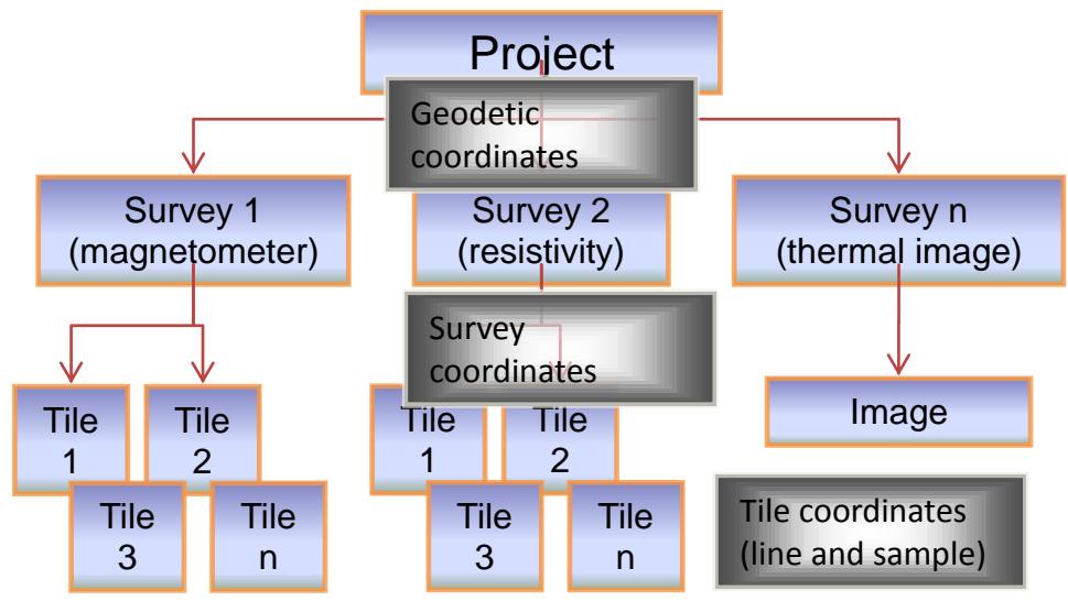
Figure 2-6. Project structure showing how raw data tiles are organized into surveys and surveys into projects.
