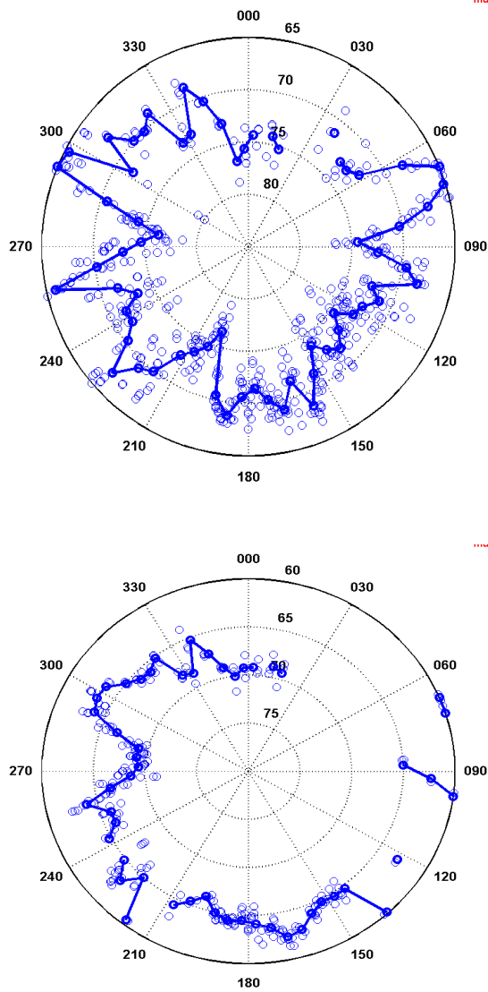
Figure 2. Top panel shows peak TL obtained from a circular track in the QPE experiment using five degree bins. Bottom panel shows integrated TL for same raw data, also using five degree binning.
