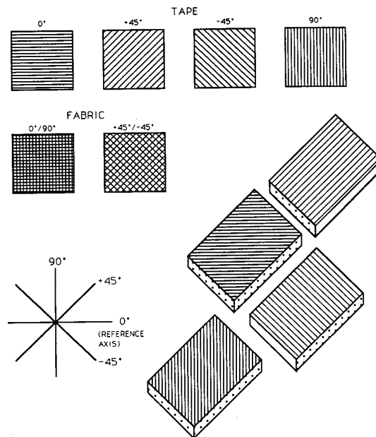
Figure 6: Lamina Fiber Orientation Code.
