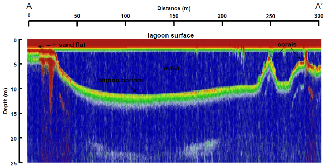
Figure 2 – 10 kHz Stratabox™ profile from A-A' on Figure 1 showing a cross section of the lagoon hollows.
