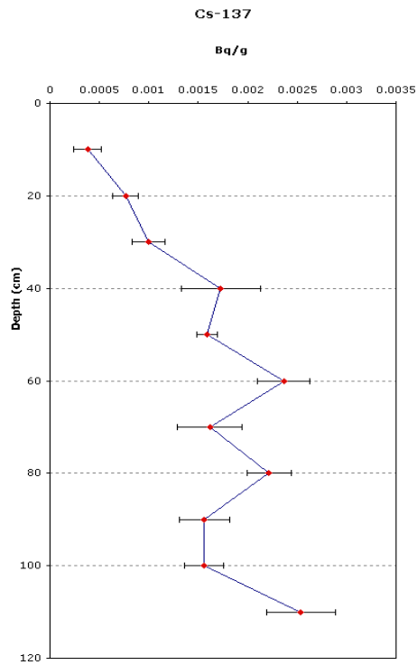
Cs-137 activity in the upper 110 cm of VC3.
