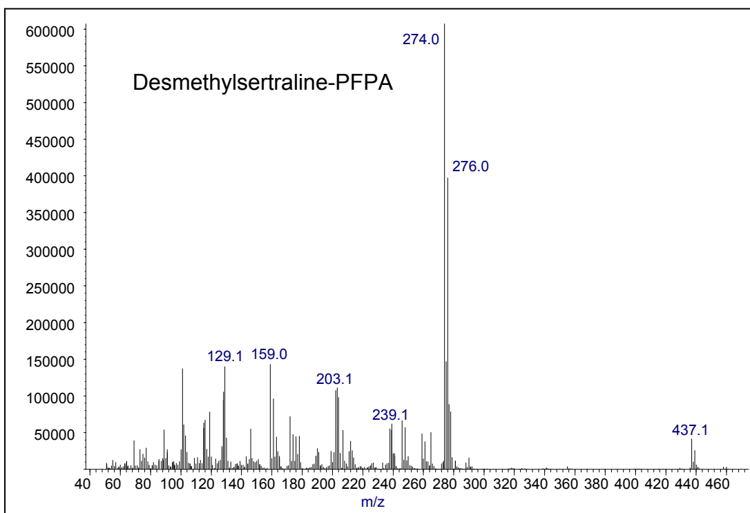
Figure 3. Representative mass spectra for desmethylsertraline (PFPA derivative).
