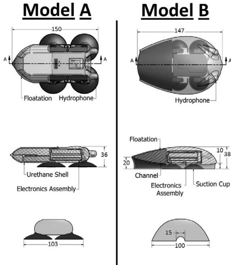
Figure 9 First column : Model-A tag geometry along with the largest cross section of the housing when the package is aligned with the direction of the flow (lower-left). Second column : Model-B tag geometry along with the largest cross section of the housing when the package is aligned with the flow (lower-right). A streamlined half-body provides a skirt around the cups to minimize geometric disruptions to the flow. All dimensions are in millimeters.
