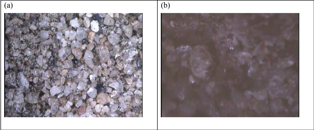
Figure 21. Digital images with the dual-camera system to test lighting, (a) sand soil at a 6.4-mm field of view, and (b) sand soil at a 1.7-mm field of view.
