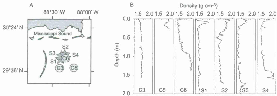
Fig. 5. (A) Locations of bottom samples collected before (circles) and after (stars) Hurricane Katrina. (B) Density profiles of cores. Pre-Katrina cores C3 and C6 have densities of \sim 1.5 \text{ g cm}^{-3} at the seafloor, whereas the post-Katrina cores (S1–S4) have values above 1.7 \text{ g cm}^{-3} . Note that core C5 also has a higher density because it is near the edge of the extensive sand sheet to the east. The deepest evidence of the Katrina bed is in core S2, which shows a spike of sandy (density \approx 1.7 \text{ g cm}^{-3} ) sediment at 0.58 m. The full dataset is presented in Furukawa et al. (2006). The sand that is present in the upper 0.5 m of the post-Katrina cores was probably transported from the sand sheet by southwestward currents as observed for Hurricane Ivan (Teague et al. , 2006b).
