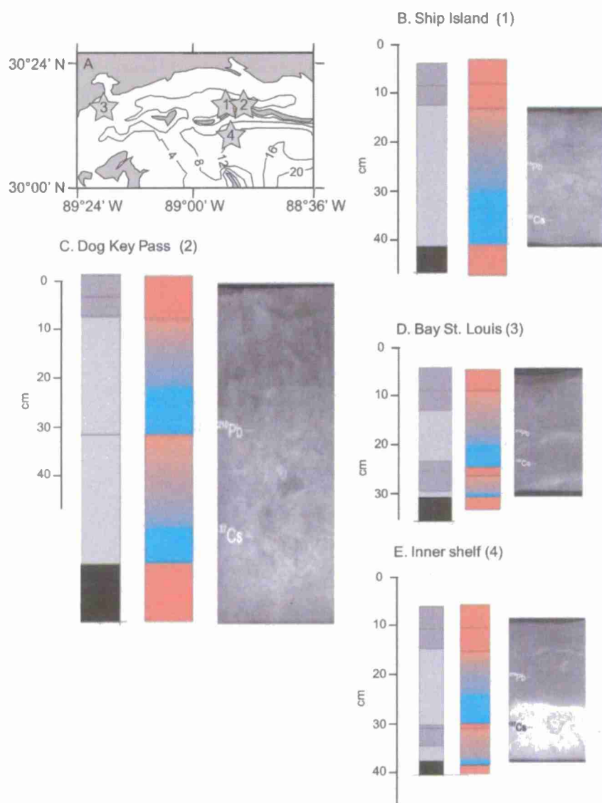
Fig. 8. Storm beds within Mississippi Sound for a 1947 hurricane and Hurricane Camille (1969). (A) Location map for cores discussed in text and this figure (location shown in Fig. 3). Synthetic cores (left column), synthetic cores with bioturbation (middle column) and x-radiographic negatives of real cores for the Mississippi Bight: (B) Ship Island; (C) Dog Key Pass; (D) Bay St. Louis; and (E) the inner shelf. The synthetic cores contain pre-storm mud (black), storm beds (light shade) and fair-weather mud (darker shade). The degree of preservation of the original fabric for the bioturbated synthetic cores is indicated by colour; blue is original fabric and red is completely disrupted (Keen et al. , 2004). ^{210}\text{Pb} and ^{137}\text{Cs} represent core dating presented in Keen et al. (2004).
