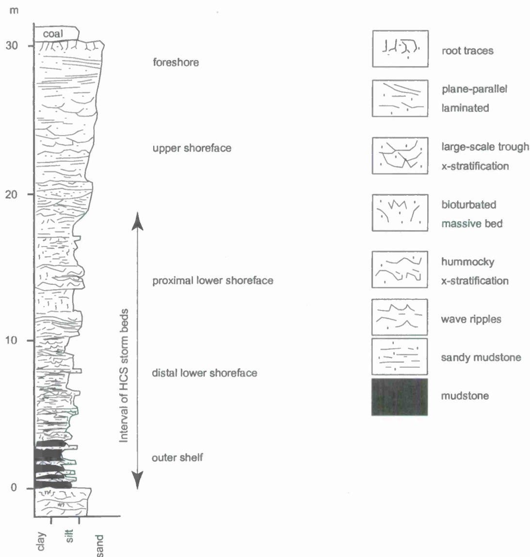
Fig. 10. Graphic log of the Campanian-age Sowbelly parasequence, Spring Canyon Member, Blackhawk Formation in Gentile Wash, Utah (39°42'56.31" N; 110°52'28.74" W). The sequence was deposited as a storm-dominated sandy shoreline prograded approximately 10 km ESE over approximately 100,000 years. Approximately 75 identifiable discrete hummocky cross-stratified (HCS) storm beds are preserved in the section.
