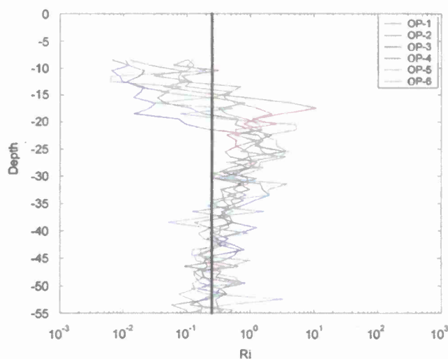
Fig. 7. The median gradient Richardson number profiles in the water column at Station B90 during the different observational periods, as determined from ADCP and MSS measurements. The thick line corresponds to Ri value of 0.25.
