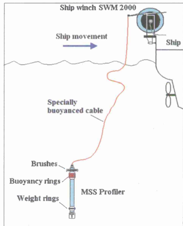
Fig. A1. Sketch of the apparatus employed during the turbulence measurements.
