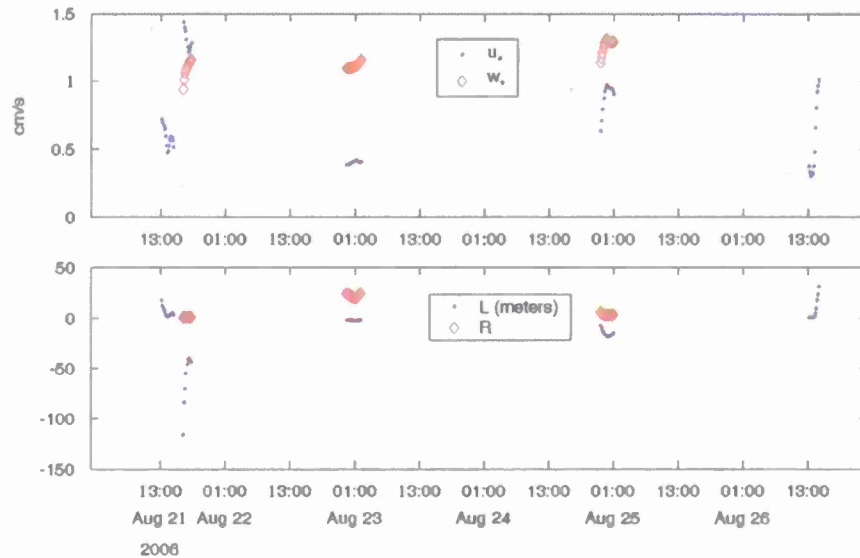
Fig. 4. Friction velocity u_w and convective velocity scale w_c (cm/s, top panel); Monin–Obukhov length scale ( L , meters) and the non-dimensional ratio R = (w_c/u_w)^3 (bottom panel) during the 6 observational periods of microstructure measurements at Station B90. The OPs are from left to right OP-1, OP-2, OP-3, OP-4 and OP-5/6.
