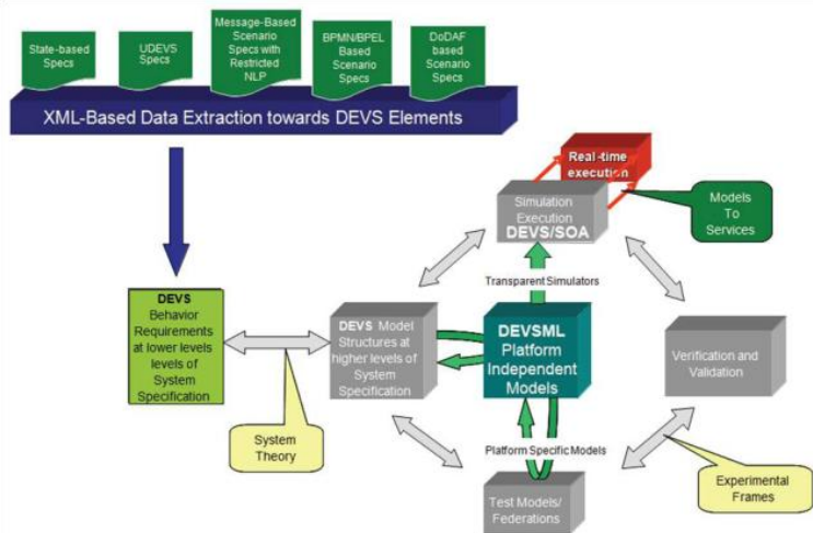
Figure 5. DEVS Unified Process
