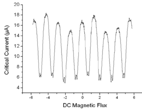
Figure 10. The dependence of the critical currents of the two-cell SQUID on the externally applied DC magnetic flux.
