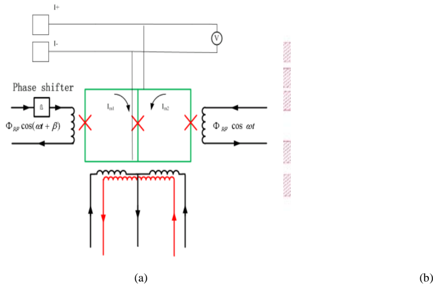
Figure 15. (a) The sketch and (b) the layout of the two-cell SQUID circuit.
