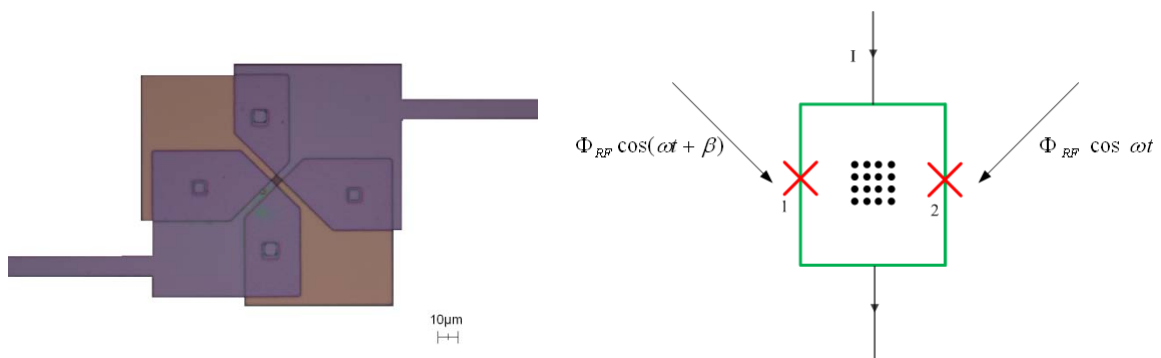
Figure 4. (a) The optical image of the one-cell SQUID circuit with two JJs.
