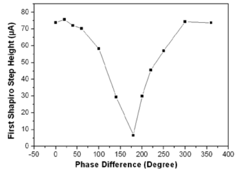
(b) The dependence of the height of the first Shapiro step of the one-cell SQUID on the phase difference of two microwave radiation signals.
