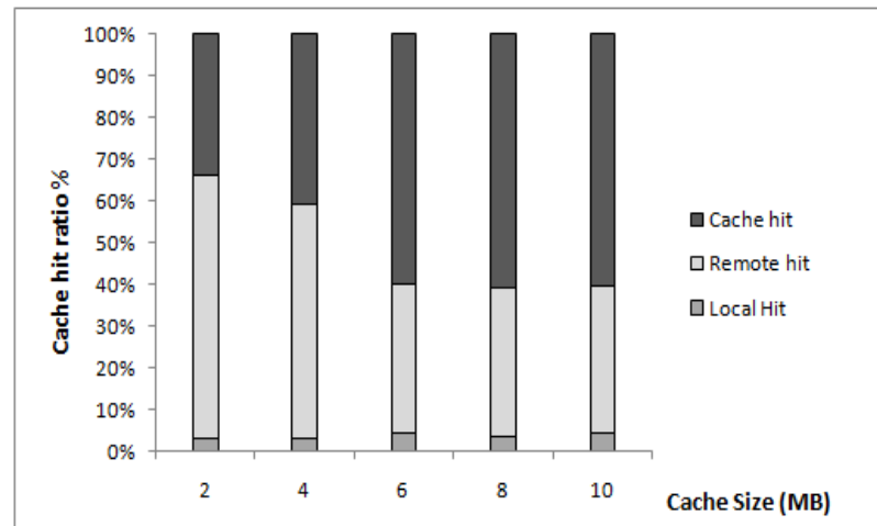
Figure 8.12b. Cache Size VS Cache Hit Ratio % ( DGA)
