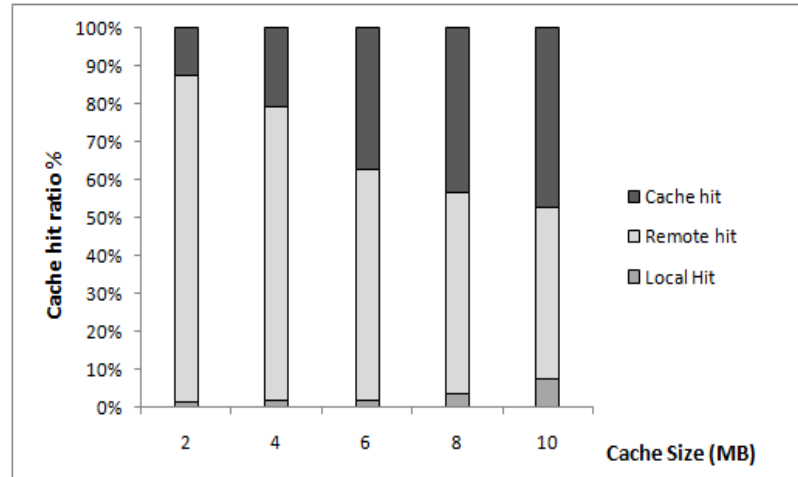
Figure 8.12a. Cache Size VS Cache Hit Ratio % ( MELOC-X)
