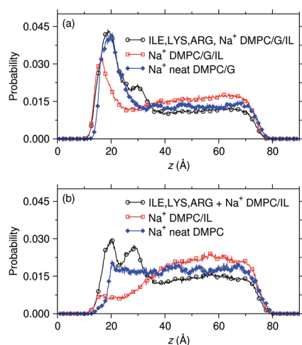
Figure 9. Distributions of \text{Na}^+ and positively charged residues in the presence and absence of indolicidin. Distributions for the systems with indolicidin adsorbed onto the bilayer were calculated from configurations where the peptide was located between 20 and 27 Å away from the membrane center. The contribution from the positive charged residues of indolicidin was calculated as the sum of density distributions of the N atom at the N-terminus, the NZ atom of lysine, and the CZ atom of arginine as defined in the PDB file. (a) The total positive charge distribution for the DMPC/G bilayer including \text{Na}^+ and indolicidin charges (Ile, Lys, Arg, \text{Na}^+ DMPC/G/IL), the charge distribution due to \text{Na}^+ only in the presence of indolicidin ( \text{Na}^+ DMPC/G/IL), and the charge distribution due to \text{Na}^+ in the neat systems taken from Figure 2 ( \text{Na}^+ neat DMPC/G). (b) The same distributions for the DMPC bilayer.
