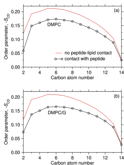
Figure 10. Order parameter -S_{\text{CD}} along the lipid acyl chain of (a) DMPC and (b) DMPC/G bilayers calculated with eq 1. The carbon atoms are numbered sequentially from head to tail regions of a lipid. Order parameters for lipids with and without the peptide-lipid contact are represented by lines with and without circles, respectively.
