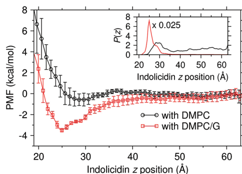
Figure 4. Potential of mean force (PMF) or free energy profiles of indolicidin as a function of the distance of the peptide from the membrane center of DMPC and DMPC/G lipid bilayers. PMF distributions with DMPC and DMPC/G lipid bilayers are shown in solid lines with circles and squares, respectively. Errors reported were based on the 95% confidence interval estimated as 1.96 times the standard error. Standard errors were estimated from the analysis of five independent PMF distributions obtained from five sets of simulations with different starting configurations of indolicidin for each bilayer. The insert shows the corresponding probability distribution P(z) of indolicidin on the two bilayers. The distribution for the DMPC/G bilayer was reduced by a factor of 40 for easier comparison with the DMPC bilayer.
