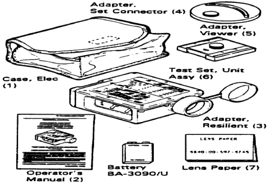
Figure 15. Electronic Test Set: TS-4348/UV (Chief, TASM-E, personal communication, April 18, 2012)
