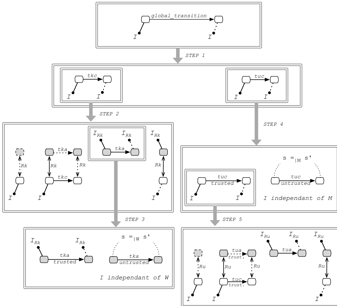
Figure 6: Structure of the locales hierarchy and proof overview.
