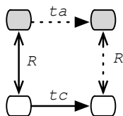
Figure 3: Forward simulation between concrete transition tc and abstract transition ta .
