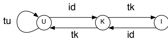
Figure 2: State automaton representing a kernel-based system.
