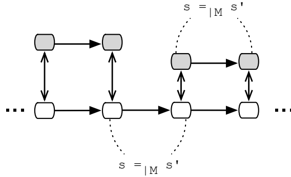
Figure 4: Schematic representation of proof decomposition.
