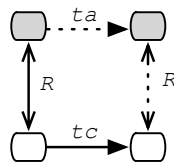
Figure 5: Forward simulation between concrete transition t_c and abstract transition t_a .
