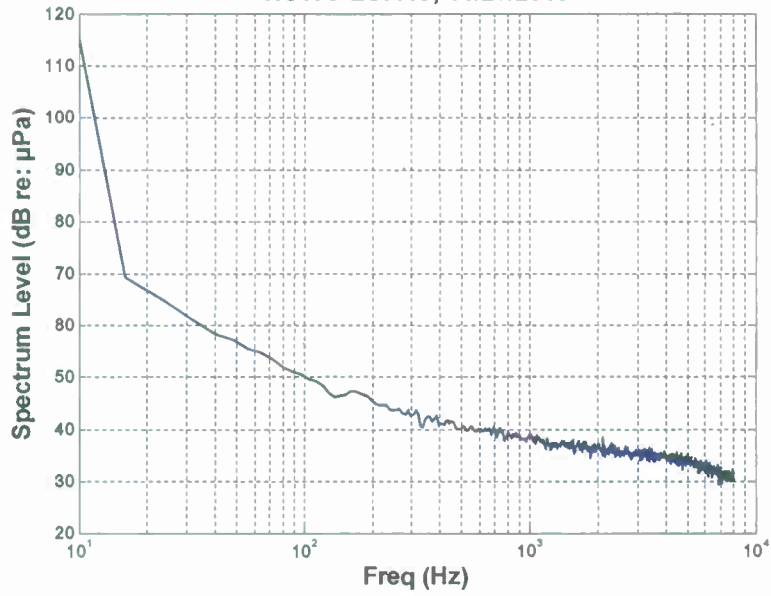
Figure 5: DMON Noise Calibration at NUWC facility, Winter 2010-2011
