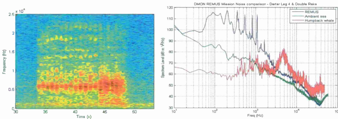
Figure 12: DMON on a WHOI REMUS Higher frequency humpback vocalization (a) frequency spectrum (b) sound level comparison
