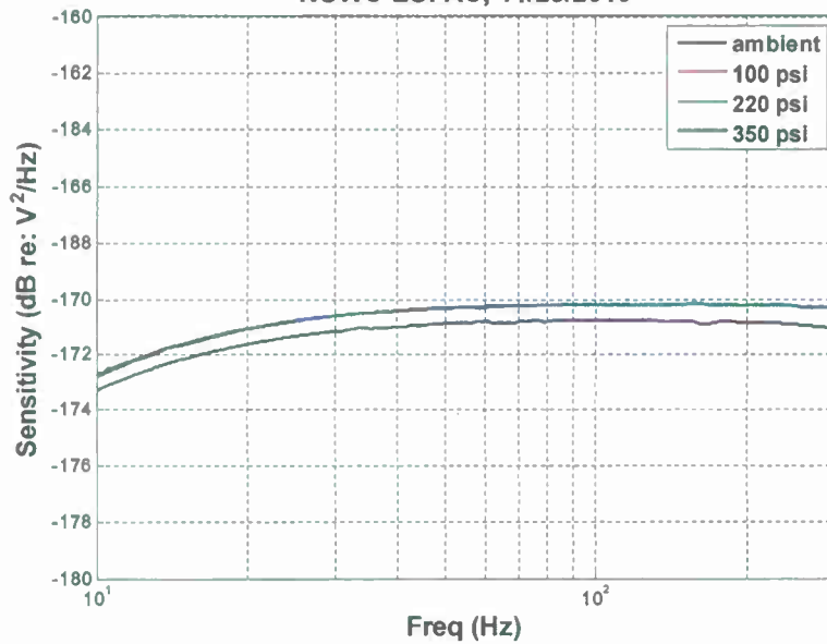
Figure 6: DMON Sensitivity at Depth Calibration at NUWC facility, Winter 2010-2011
