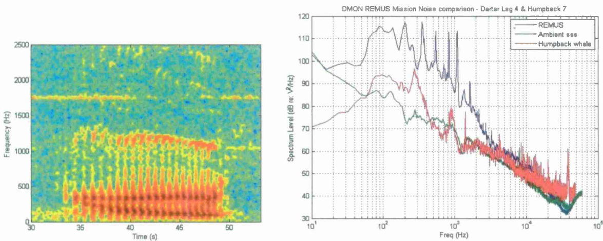
Figure 11: DMON on a WHOI REMUS Lower frequency humpback vocalization (a) frequency spectrum (b) sound level comparison
