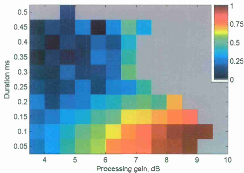
Fig. 3: Field verification of the DMON beaked whale detector in the Canary Islands. Shown is the proportion of detections considered in post-evaluation to represent an actual beaked whale click, as a function of two click parameters, energy duration and processing gain. Grey regions indicate parameter combinations for which no clicks were received. This plot helps determine how to set parameter thresholds for beaked whale classification. For example, choosing a processing gain threshold of 4+10 \times \text{duration} (in ms) eliminates many false detections.
