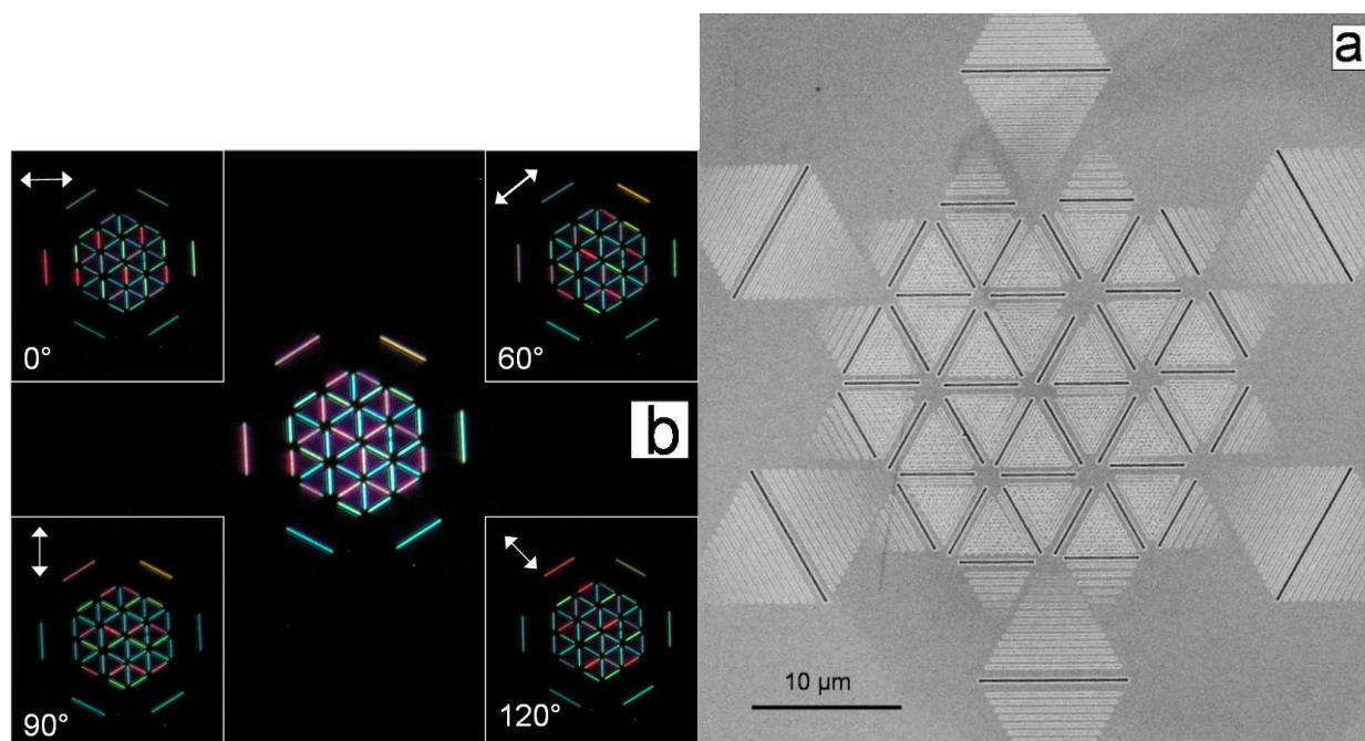
Figure 4 Polarization response of slit-groove lattice. a, SEM image of a 2 D lattice with downsized slits (length 5 \mu m, width 170 nm) with grooves (width 150nm, linear depth gradient from 150nm to 10 nm) for 3 periods (450, 500 and 580nm) surrounded by slits of length 10 \mu m with periods varying from 450 nm (blue) to 580 nm (red). b, Microscope picture of this structure when illuminated with unpolarized light (center) and polarized light (boxes). The overall illuminating intensity is weaker for the polarized images due to the attenuation of the polarizer.
