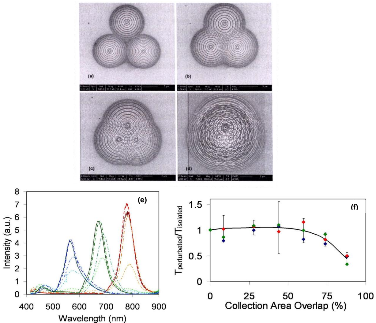
Figure 2 Photon sorting efficiency of triple bull's eye structure. a to d.: Triple bull's eye structures with periods 530 nm, 630 nm and 730 nm, fabricated with different degree of overlap. e: Transmission spectra measured at each hole as a function of structural overlap (bold lines separated bull's eye structures, dashed line 44% overlap, dashed-dotted 77%, dotted lines 88%). The depth parameters are the same as in Figure 1a. f: Transmission peak intensities normalized to the isolated bull's eye peaks shown in b as a function of overlap. The error bars reflect the spread in measured values for 6 data points and the points the average for each colour peak.
