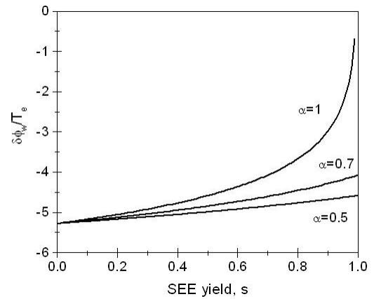
Figure 14 – Dependence of the sheath potential drop on wall material SEE yield.
