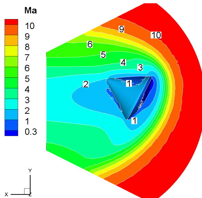
Figure 4a: Contours of Mach number about a capsule at angle of attack [30].
