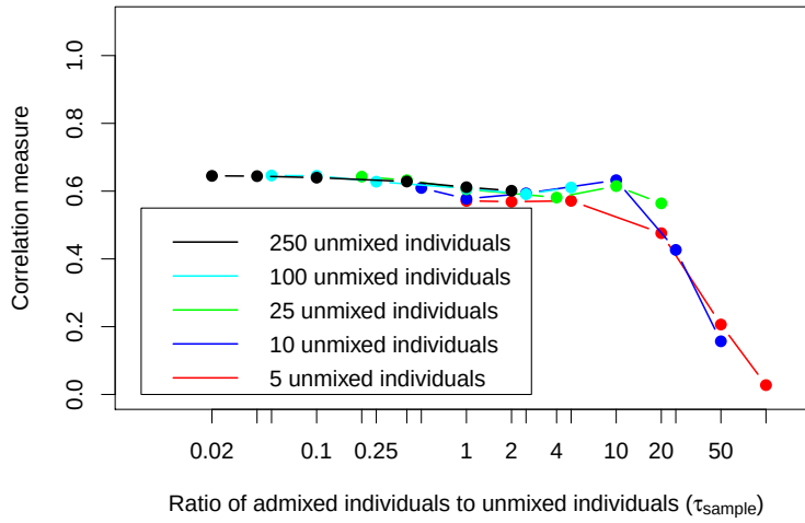
(b) Using Eigensoft
