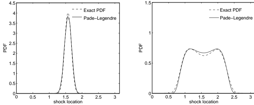
Figure 14: Probability distribution of the shock location for the inhomogeneous Burgers equations with uncertain initial condition. Low \sigma , \sigma = 0.1 (left) and high input variability, \sigma = 0.6 (right). Results obtained using the Pade-Legendre stochastic collocation approach [32]
