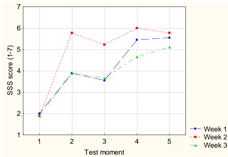
Figure 16: SSS score
