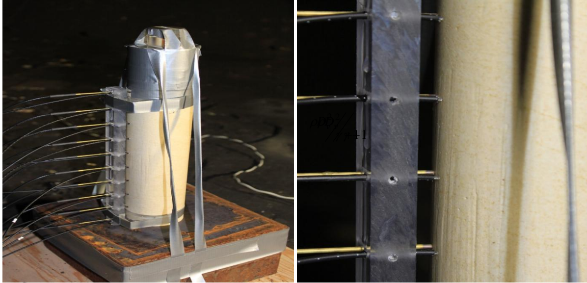
Figure 1: Images of the experimental setup for the determination of detonation velocity (left) and a close up image (right) of the fiber optic and piezoelectric pin holder design.
