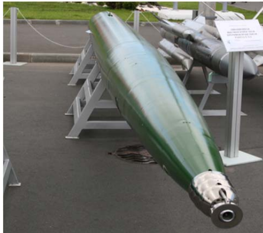
Figure 17. VA-111 Shkval Super-Cavitation Rocket-Propelled Torpedo From [57]
