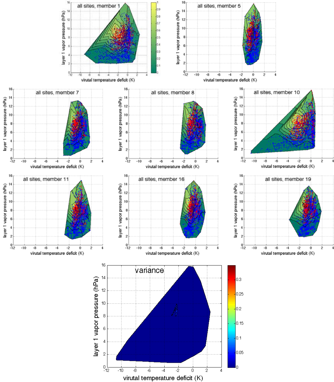
Figure 84. Observed fog (red) and no fog (blue) plotted in the all regions domain joint parameter space of JP\_B for each member. Contouring is based on bin sizes equaling one-twelfth of the total data in each plot. The variance of the probability output among all the plots is shown in the bottom panel. The first six hours of each case are excluded.
