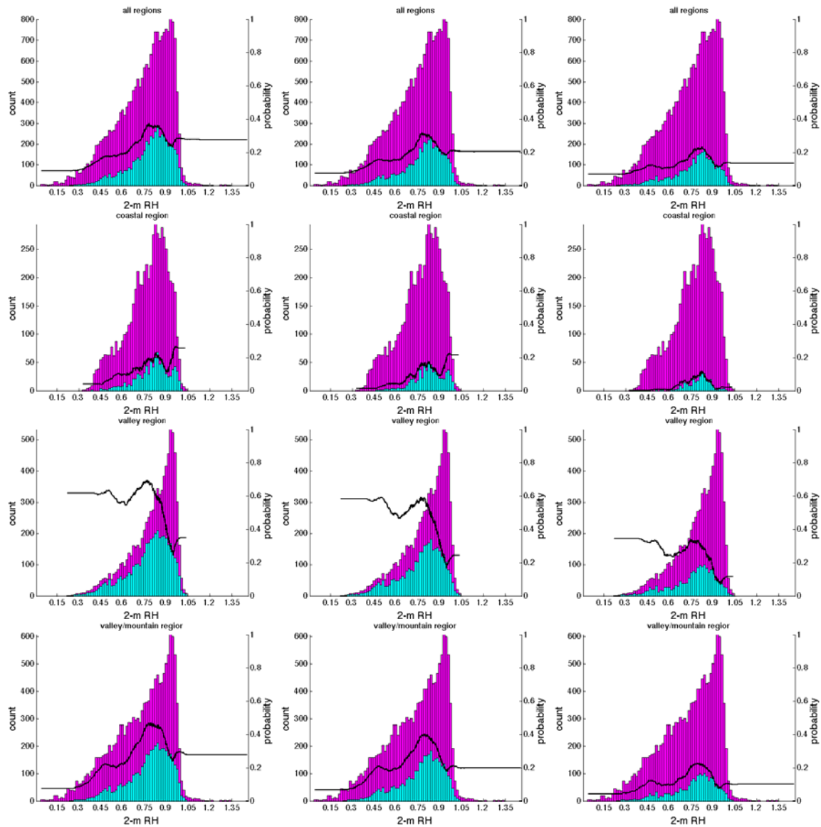
Figure 69. Same as in Figure 68, but with the light blue portion of the distributions and the output probability of exceedance corresponding to each of the three other \beta_e thresholds: 0.41 km -1 (left column), 0.68 km -1 (center column), 2.10 km -1 (right column). The rows correspond to each of the four domains: all regions (top row), coastal region (second row), valley region (third row), and valley/mountain region (bottom row). The first six hours of each case are excluded.
