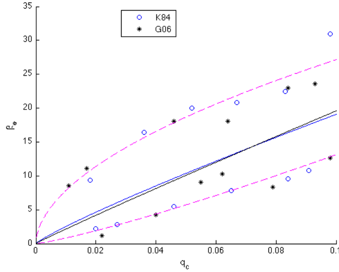
Figure 9. Plot of selected data from Kunkel (1984) and Gultepe et al. (2006). The two solid lines through the middle are regression lines for each data set, and represent the Stoelinga and Warner (1999) visibility parameterization (blue) and the Gultepe et al. (2006) visibility parameterization (black).
