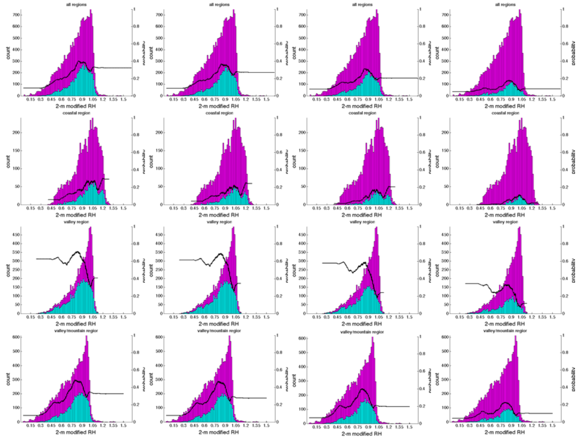
Figure 70. Same as in Figure 68 and Figure 69, but after a 2-m temperature bias correction has been made in the predictions. The columns correspond to each of the four \beta_e thresholds, increasing from left to right. The rows correspond to each of the four domains: all regions (top row), coastal region (second row), valley region (third row), and valley/mountain region (bottom row). The first six hours of each case are excluded.
