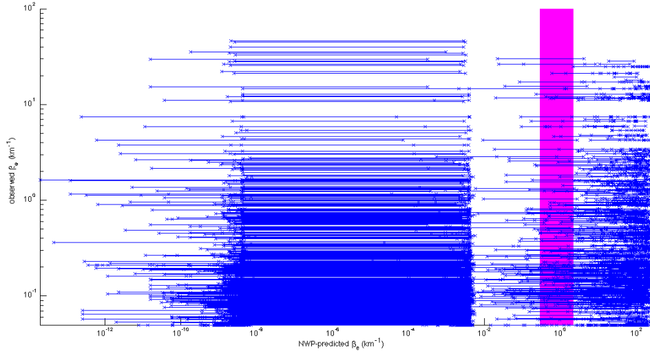
Figure 20. Scatter plot of observed versus NWP-predicted \beta_e for all members. Each prediction is plotted as a blue segment, which indicates the range \bar{\beta}_e \pm 3\sigma from the parametric visibility parameterization. The pink box indicates the approximate range of \beta_e values corresponding to light fog.
