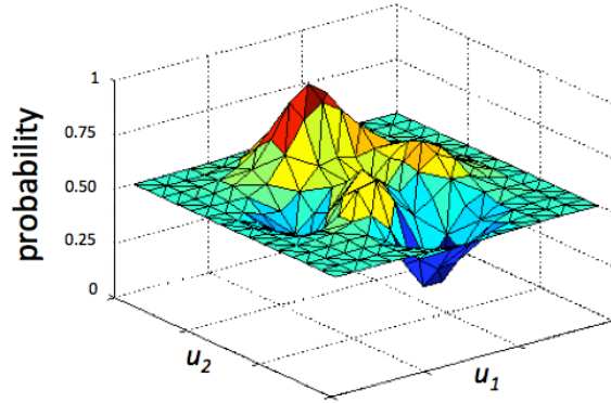
Figure 73. Notational illustration of Dulauney triangulation in the two-dimensional joint parameter space u_1, u_2 . In this example the probability forecast values plotted on a third axis to aid in the conceptual visualization of the interpolation scheme. (After The Mathworks, Inc. 2009).
