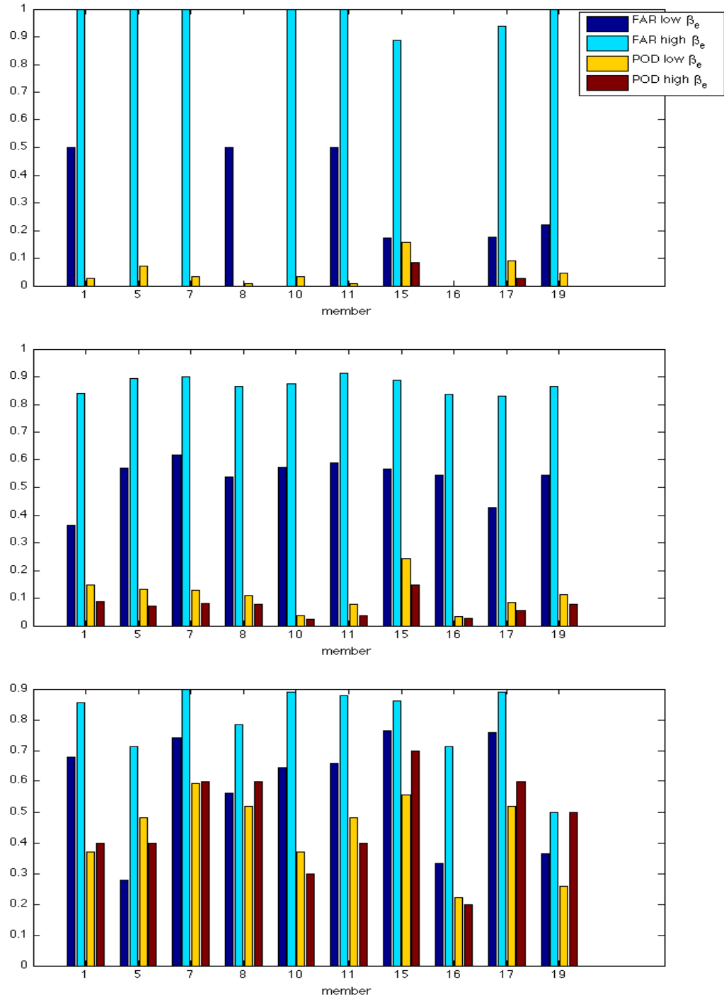
Figure 27. Comparison of false alarm ratio and probability of detection at the low \beta_e threshold ( 0.29 \text{ km}^{-1} ) and high \beta_e threshold ( 2.1 \text{ km}^{-1} ) for the coastal (top), valley (center), and mountain (bottom) regions. The data includes forecast hours 7-20.
