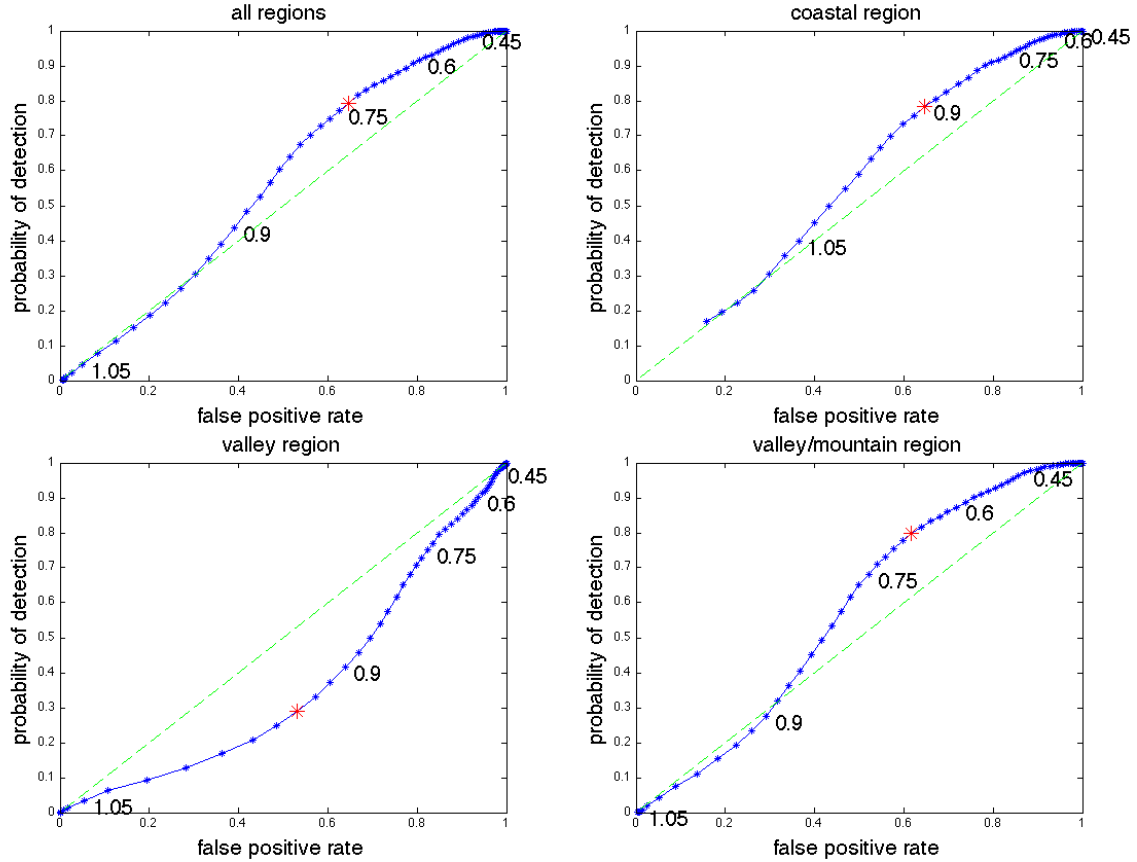
Figure 67. Same as in Figure 66, but after a 2-m temperature bias correction has been applied in each domain.
