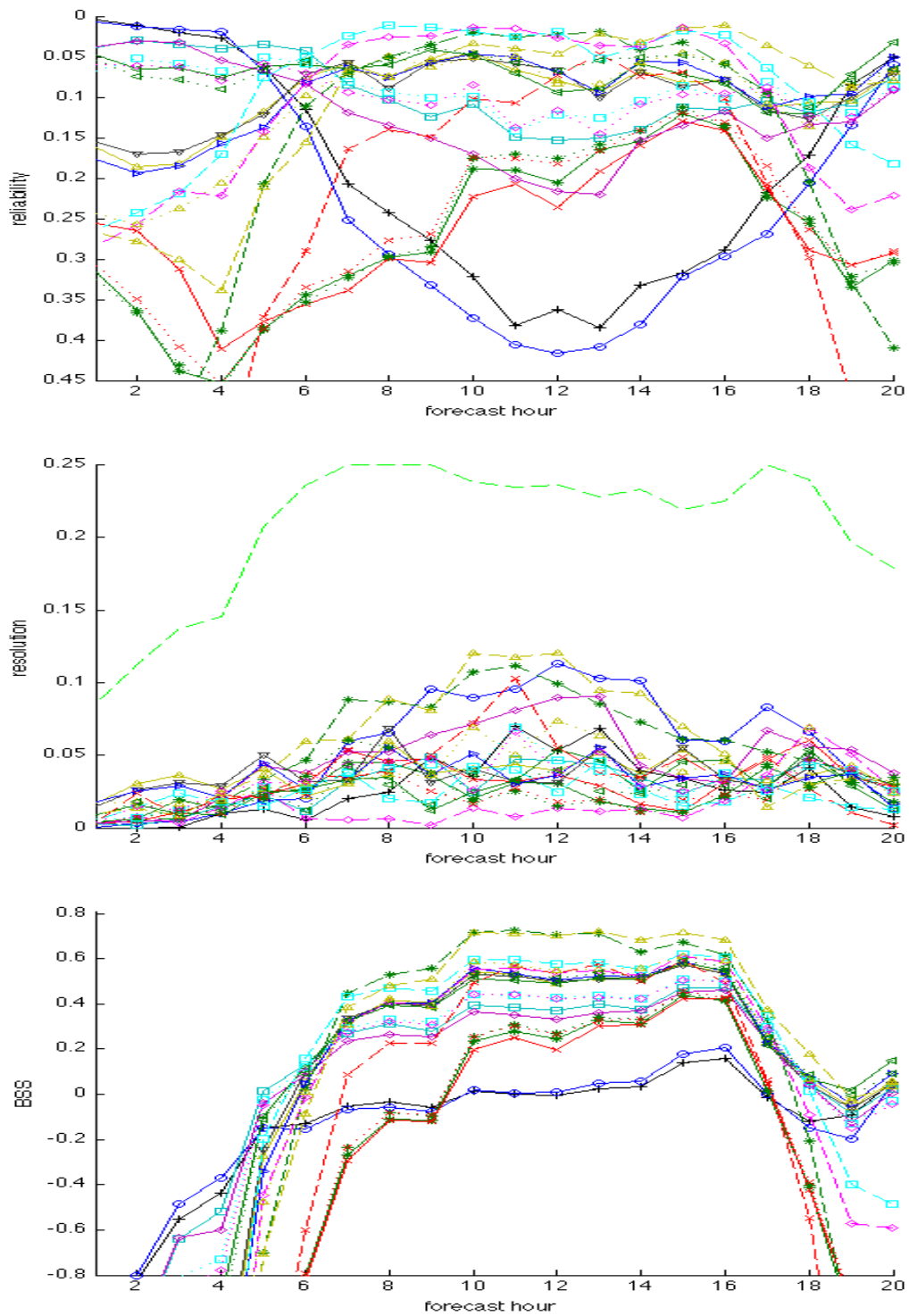
Figure 90. Same as in Figure 89, but for the valley region.
