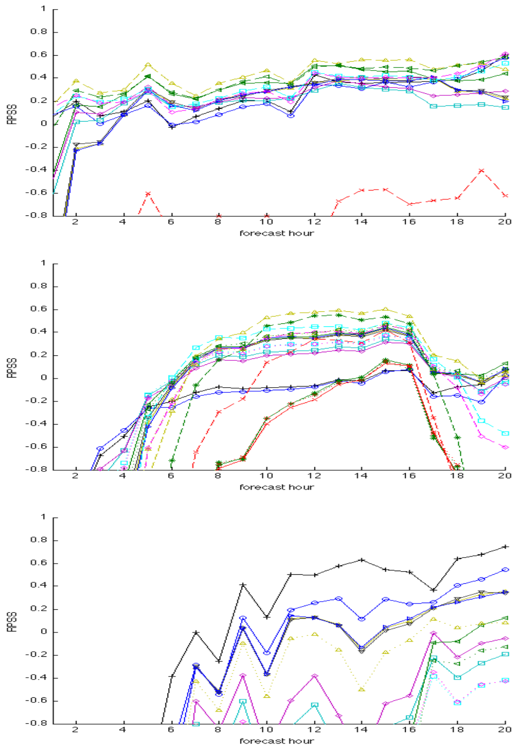
Figure 88. Same as Figure 87, but zoomed in to show more detail for the best-performing experiments.
