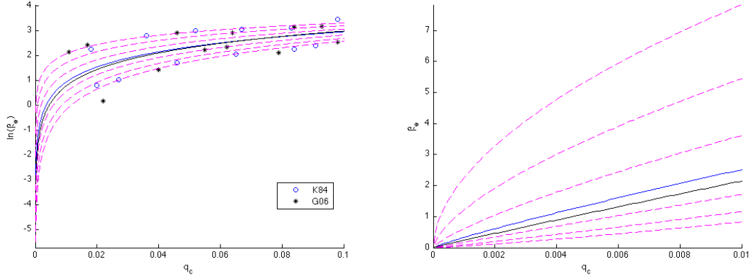
Figure 10. Left panel shows same data as in Figure 9, but plotted using \ln(\beta_e) as the y axis. The dashed lines represent one, two, and three standard deviations above and below the Stoelinga and Warner (1999) visibility parameterization (solid blue line). Right panel uses \beta_e as y-axis, and is zoomed in to show only the q_c range of interest.
