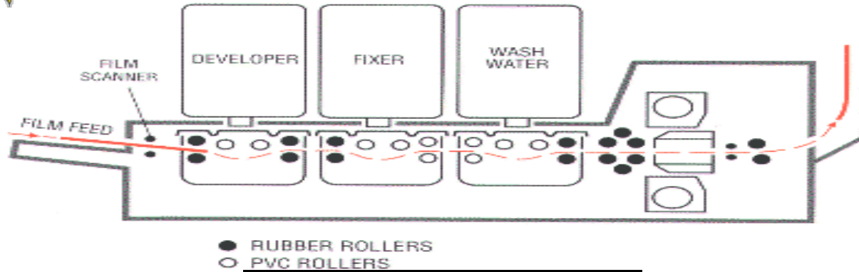
Analog X-Ray Film Processing Machine
