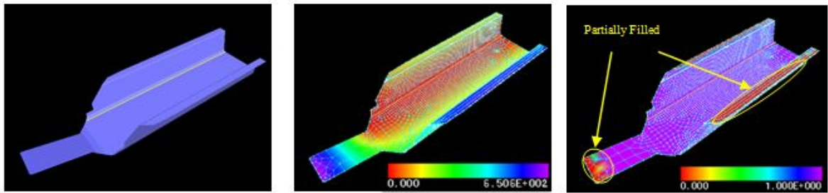
no racetracking channels, filling time = 650.6s
