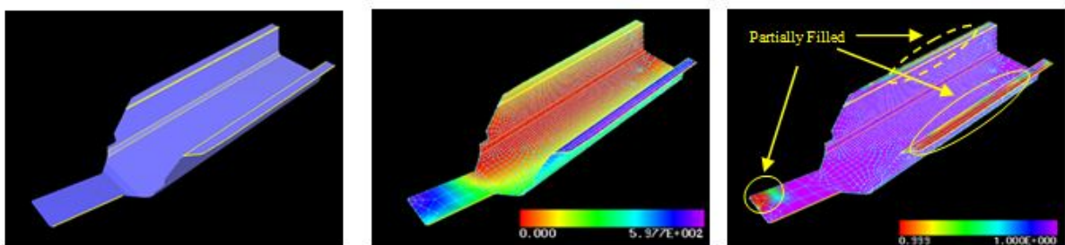
4 outer edges & 4 folds, filling time = 597.7s
