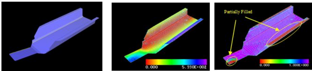
1 outer edge, filling time = 557.2s
