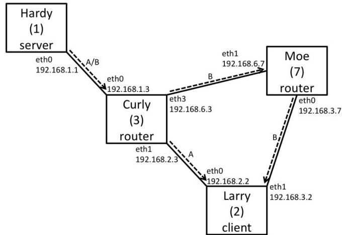
Figure 11. Test network
